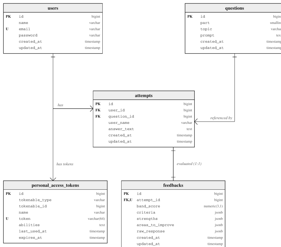
Gambar 2. Entity Relationship Diagram database aplikasi.
